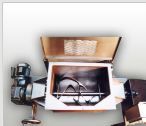
Ribbon Blenders
