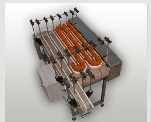
Accumulation Conveyor
